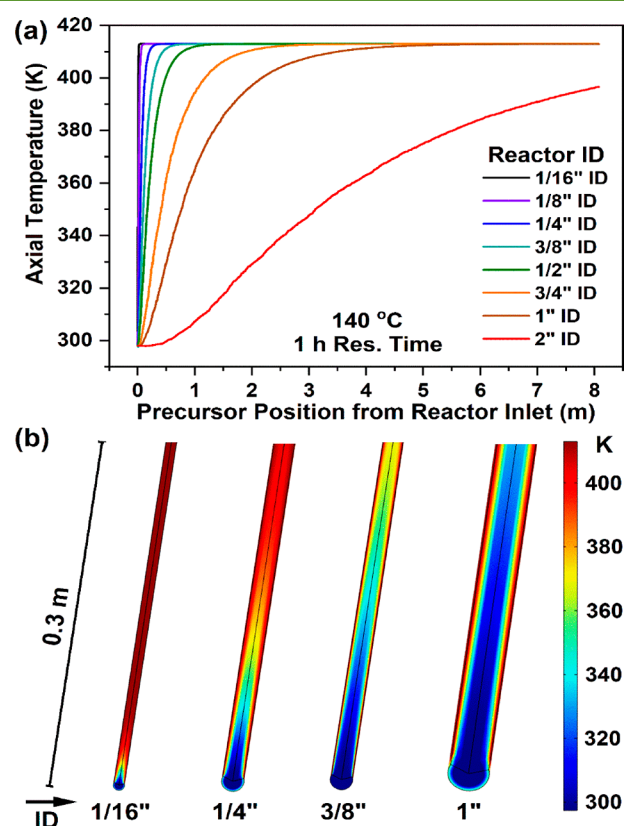
Figure 4. (a) Axial temperature profile along the length of reactor tube plotted against position of the precursor slug from reactor inlet. (b) Three dimensional (3D) slice plots at the entrance region of flow reactor showing both the temperature gradient and the growth of thermal boundary layers in the heated reaction zone as a function of tube ID. Outer diameter and tube wall is held at 140 °C, and fluid flow has linear velocity of 13.4 cm/min to achieve residence time of 60 min (8 m reactor tube length).
