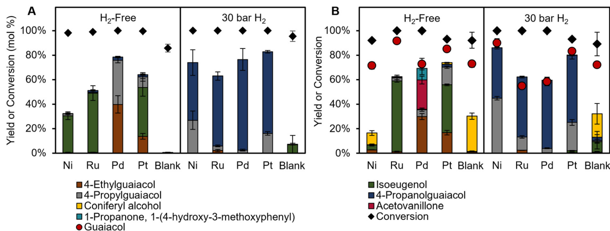
Fig. 3 Monomer product yields for model compound reactions with (A) conferyl alcohol and (B) guaiacylglycerol- \beta -guaiaicyl ether (GGE) under H_2 -free conditions (left) and with 30 bar H_2 (right). Note: for clarity, the bar for coniferyl alcohol is not shown in A. Conditions: 60 mg substrate, 20 mg catalyst, 30 mL methanol, 1 hour at 225 °C. Error bars are the standard deviation of triplicate measurements. Numerical data are provided in Tables S6–S9.†
